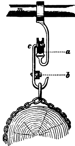
Fig. 226.—Truck.
